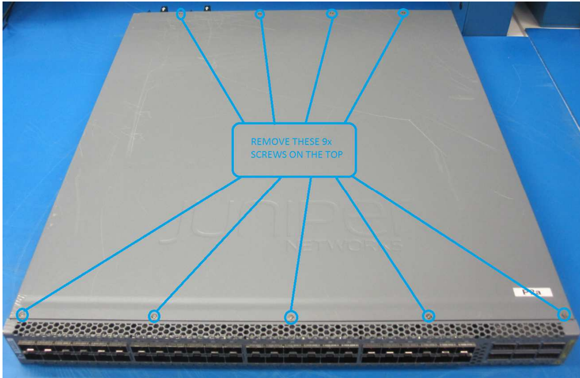
Figure 3-1: Top side screws
