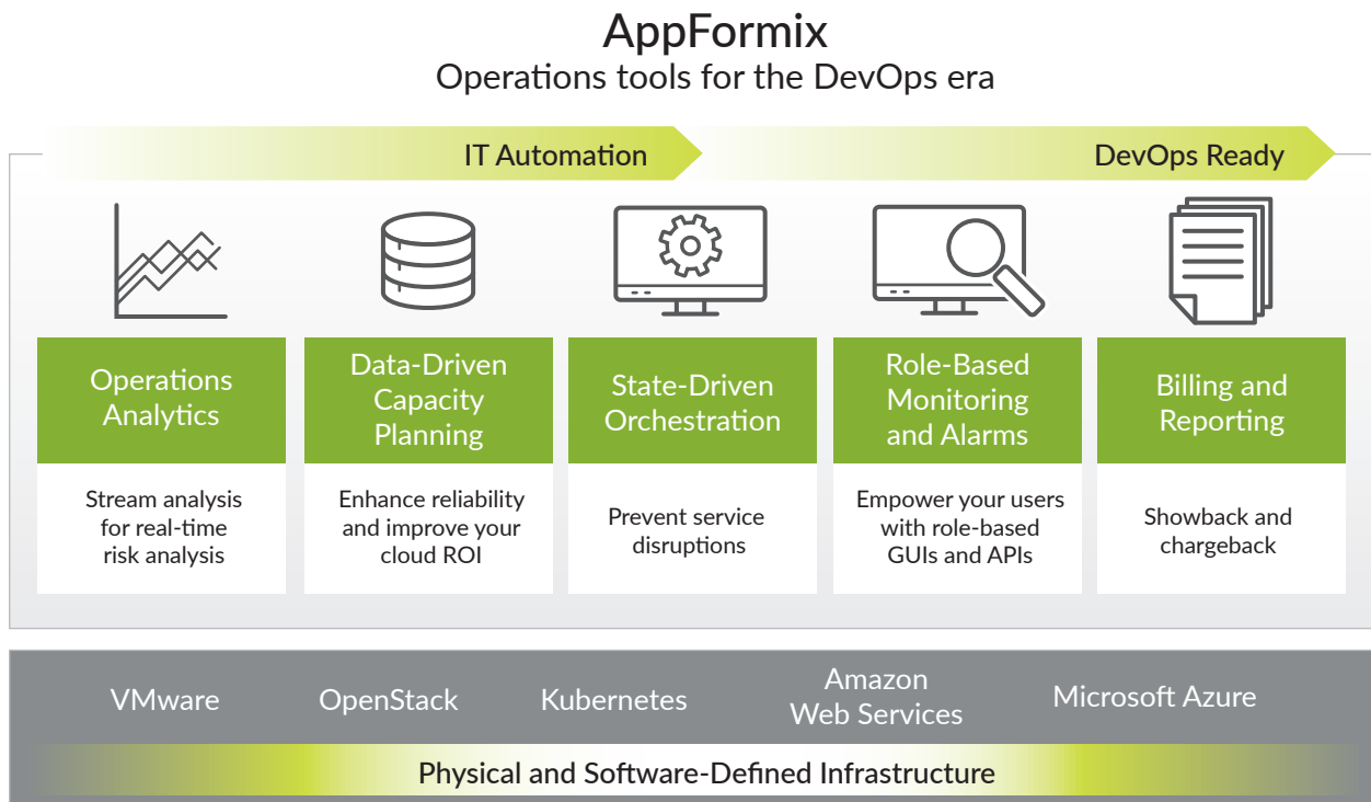
Figure 5: AppFormix overview
